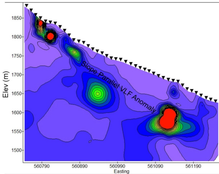
Line 4550 - VLF Profile (Seattle Transmitter)
