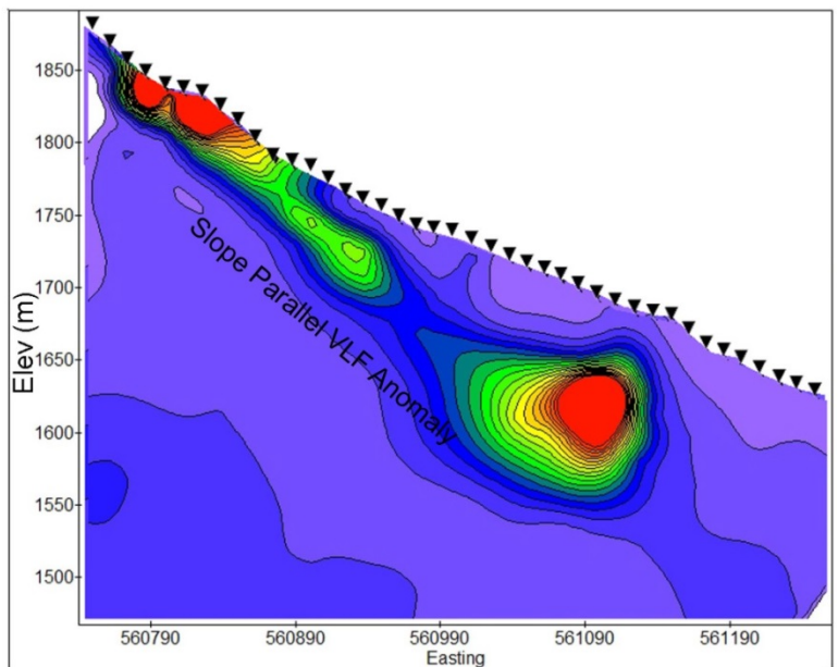
Line 4550 - VLF Profile (Hawaii Transmitter)
